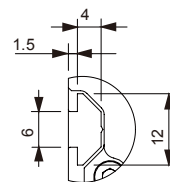
Detail Diagram C
