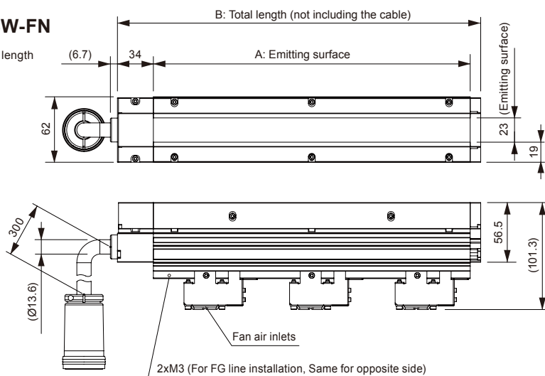
Mounting slot 4, nut slots See "Detail Diagram C".
