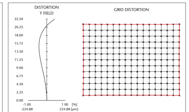
ML-3528-43F DISTORTION DIAGRAM
