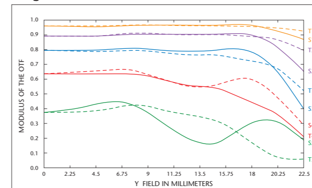
ML-3528-43F MTF VS. FIELD
